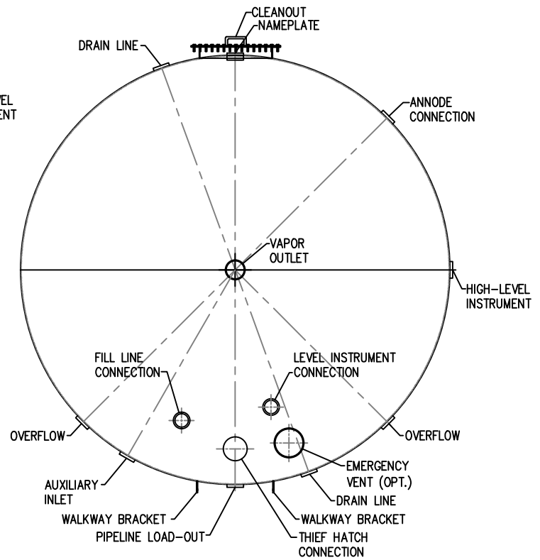
PLAN VIEW
